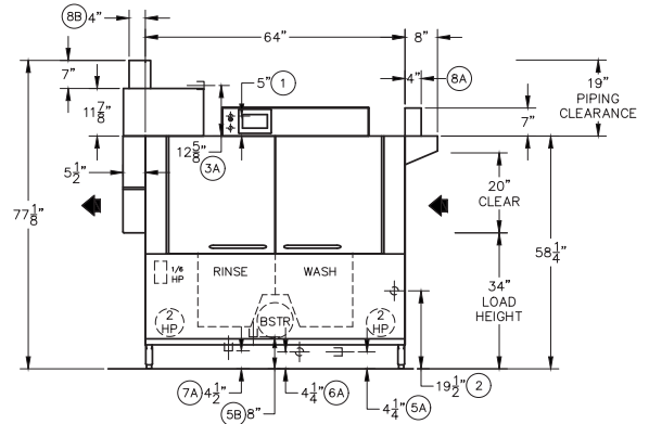
Front View: Right to Left Model R-L
