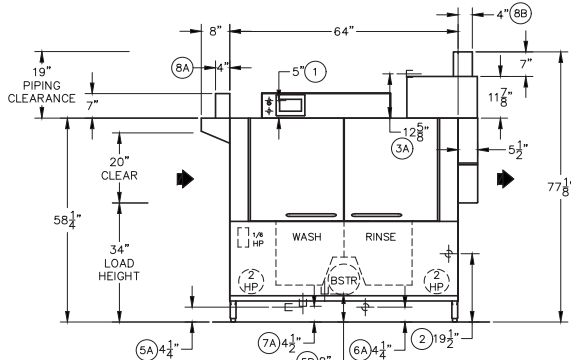
Front View: Left to Right Model L-R
