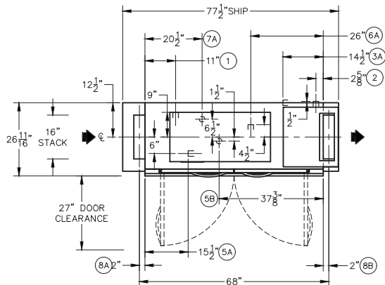
Plan View: Left to Right Model L-R
